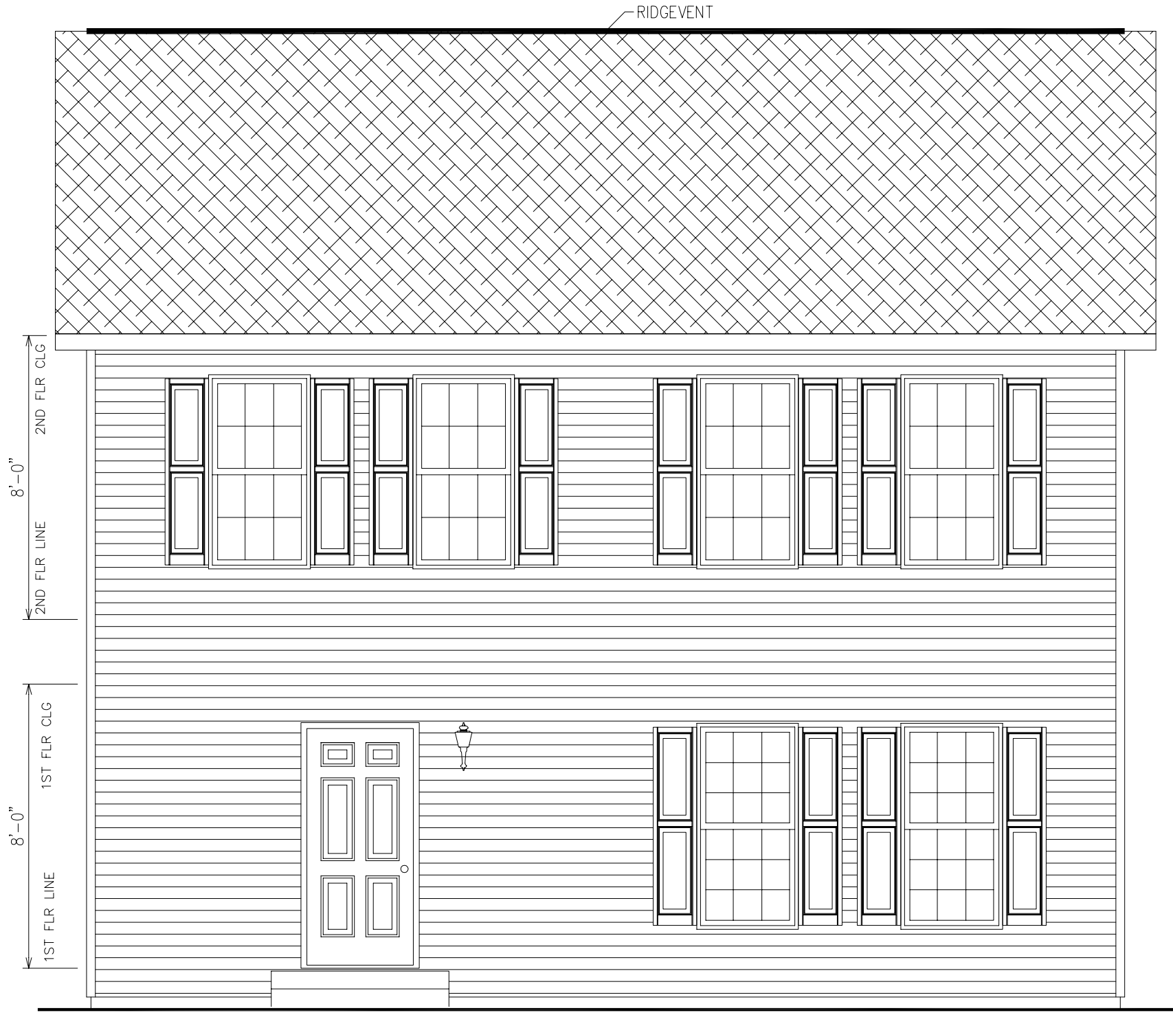
FRONT ELEVATION
