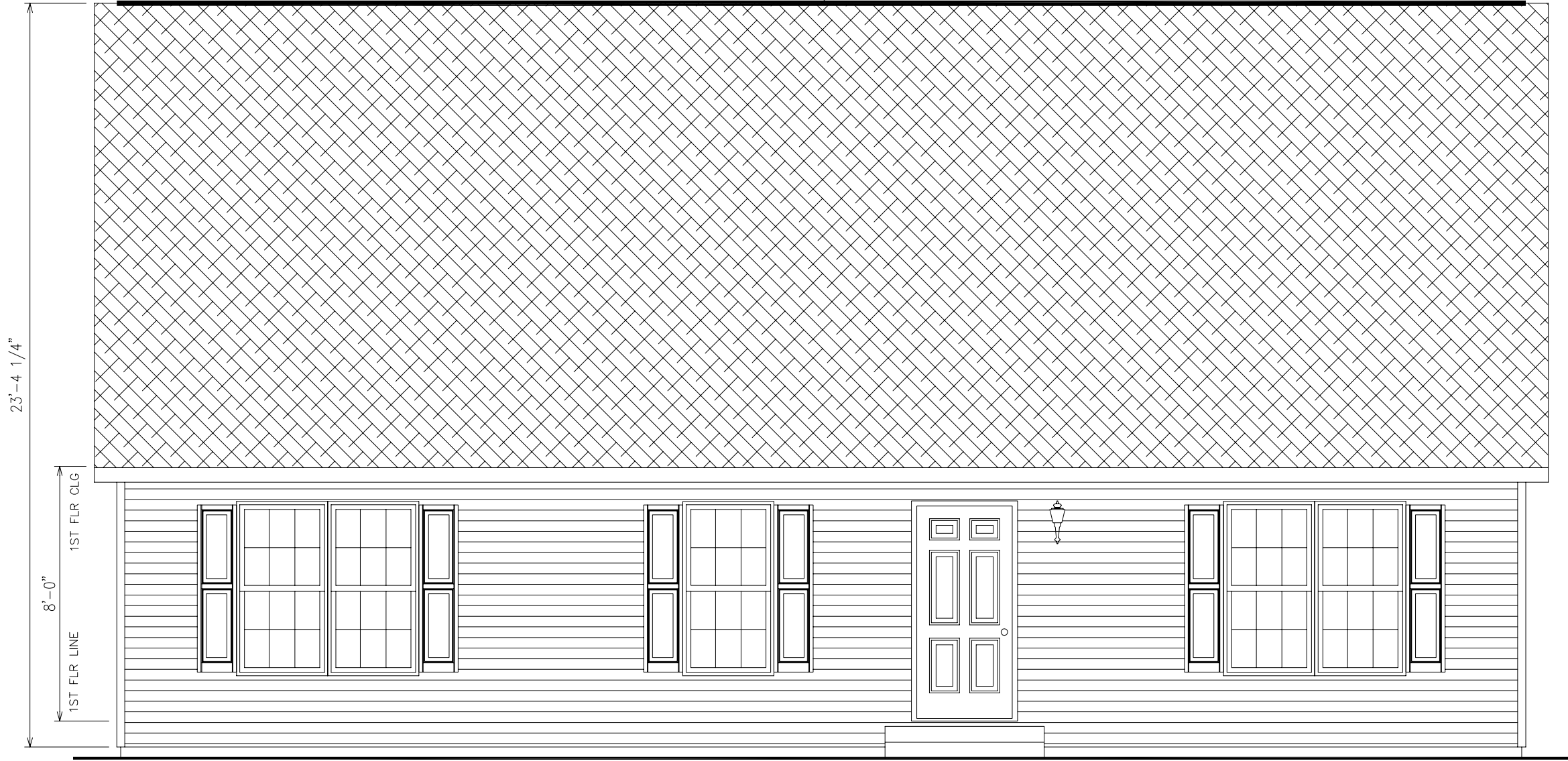
FRONT ELEVATION
